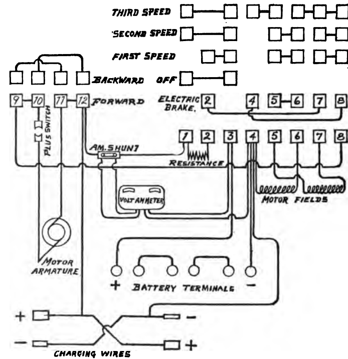
FIG. 307.—Diagram of Controller Connections of a One-unit, One-motor Circuit, with Variable Fields.
